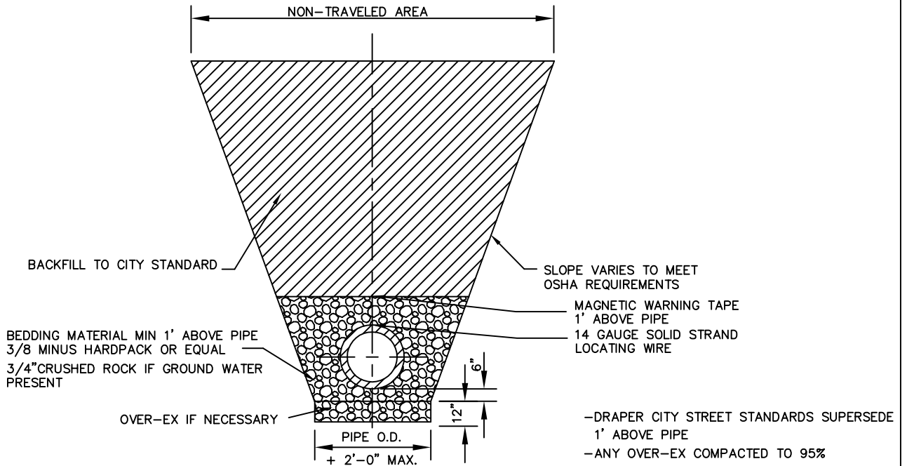
T TYPICAL NON-TRAVELED TRENCH DETAIL TYP SCALE: NONE
