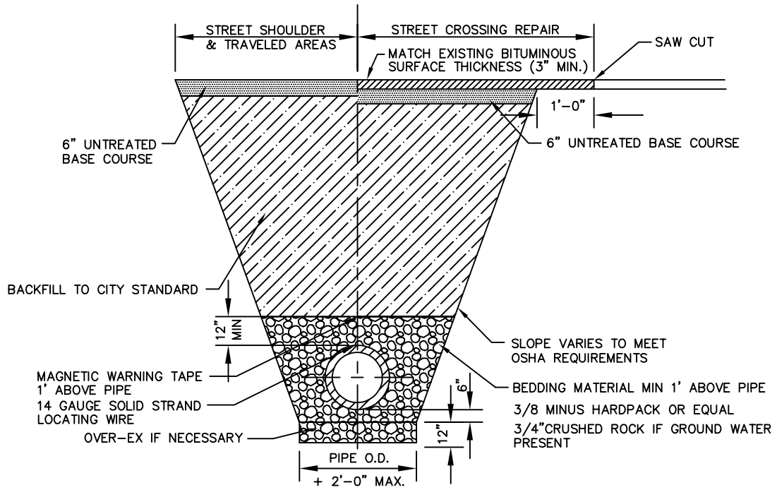
S TYPICAL STREET TRENCH DETAIL TYP SCALE: NONE
